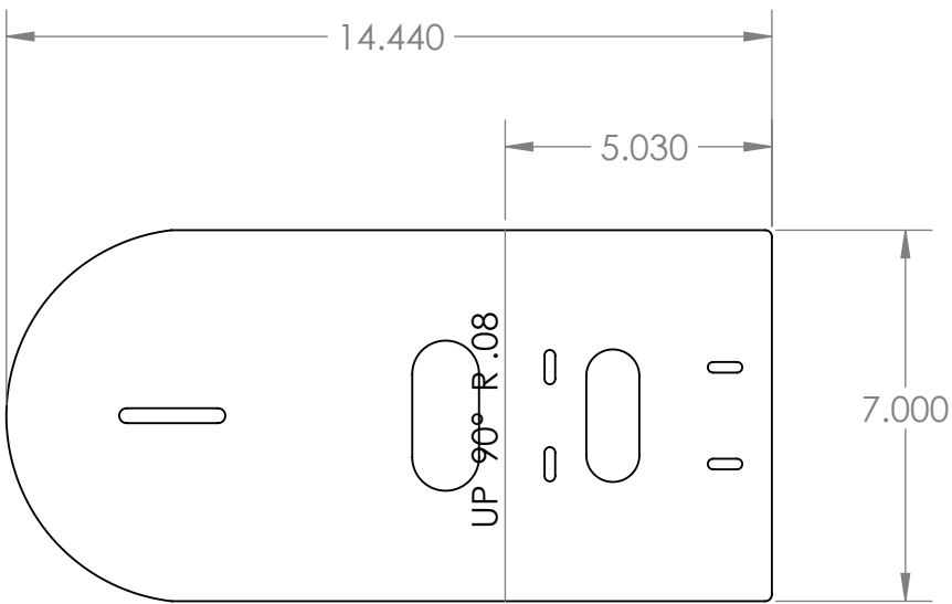
FLAT PATTERN
