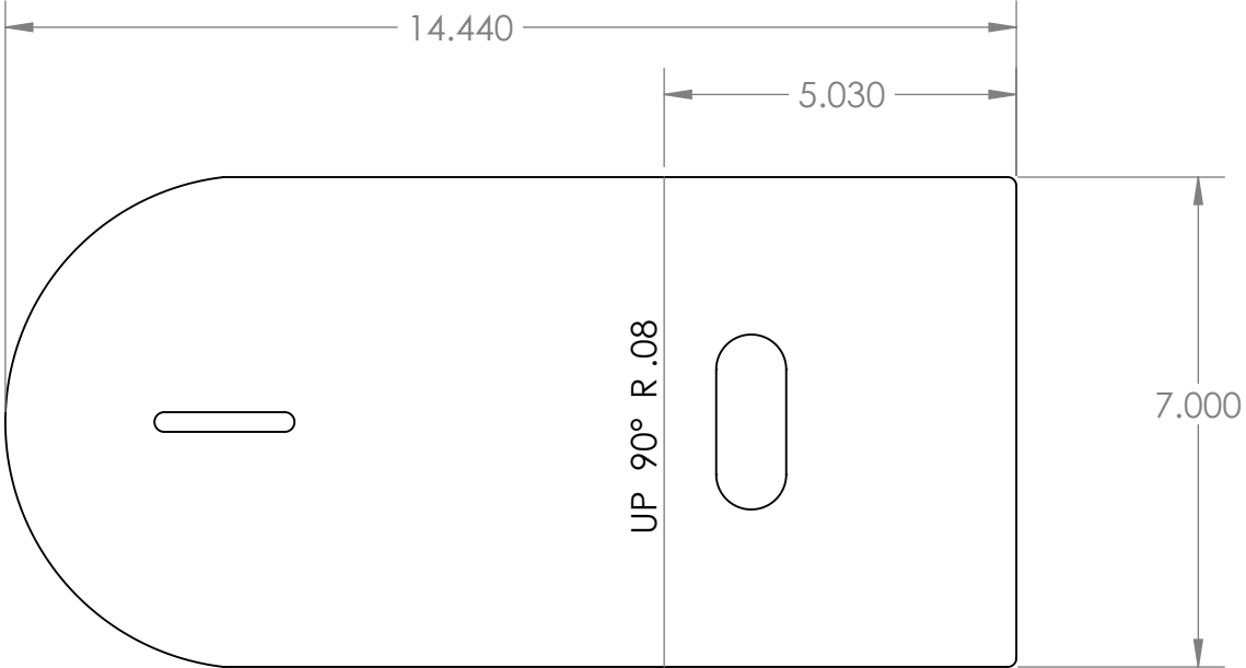
FLAT PATTERN
